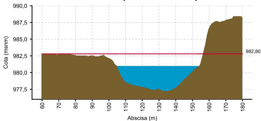
CAUCA - LA Balsa (24/04/2021 06:00 AM) NIVEL= 980.87
