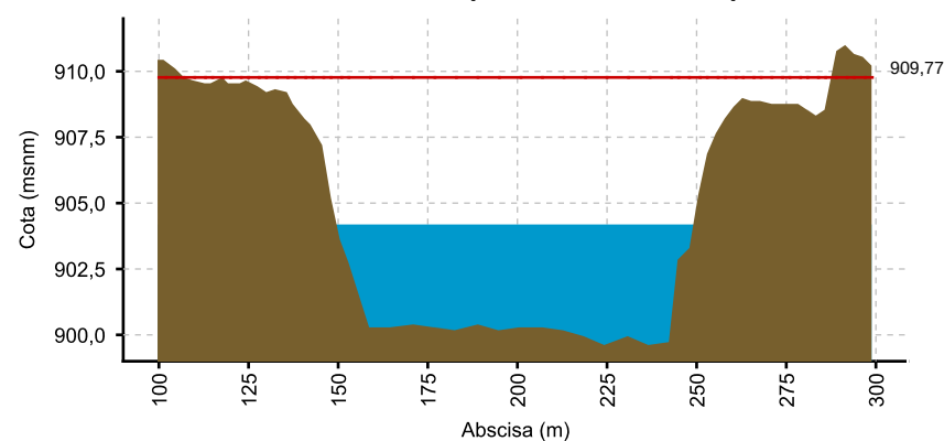
CAUCA - LA VICTORIA (24/04/2021 06:00 AM) NIVEL: 904.169
