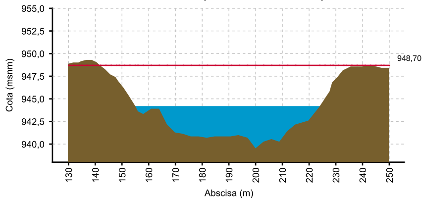
CAUCA - JUANCHITO (24/04/2021 06:00 AM) NIVEL= 944.063
