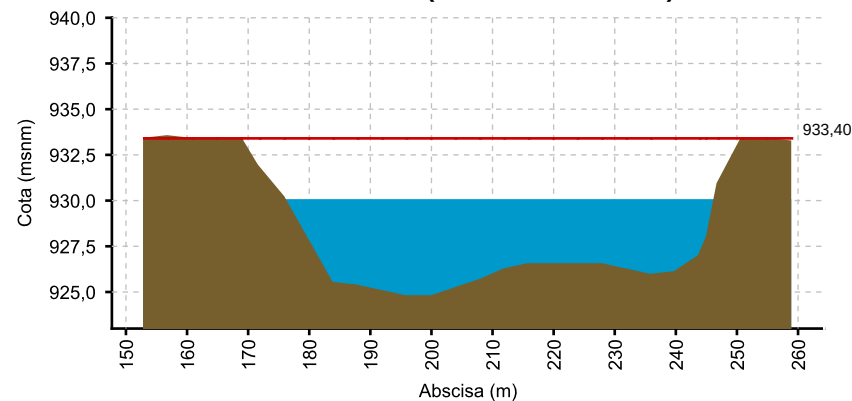
CAUCA - MEDIACANOA (24/04/2021 06:00 AM) NIVEL= 929.964
