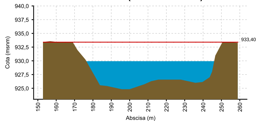
CAUCA - MEDIACANOA (26/04/2021 06:00 AM) NIVEL= 929.894
