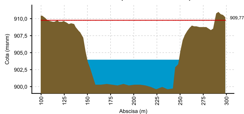
CAUCA - LA VICTORIA (26/04/2021 06:00 AM) NIVEL: 903.939
