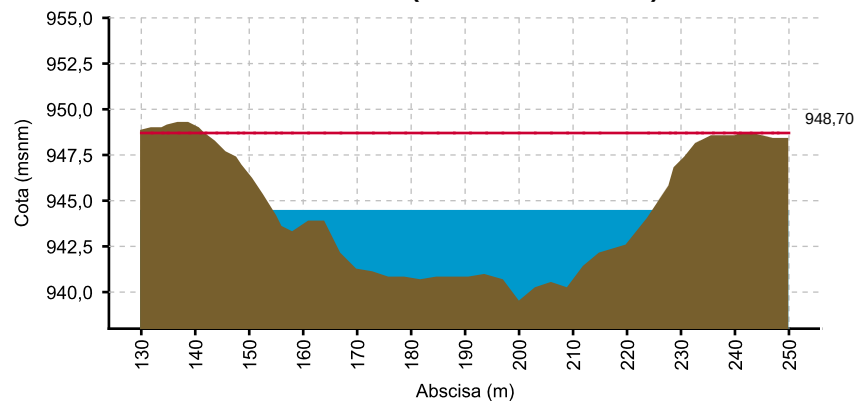
CAUCA - JUANCHITO (26/04/2021 06:00 AM) NIVEL= 944.463
