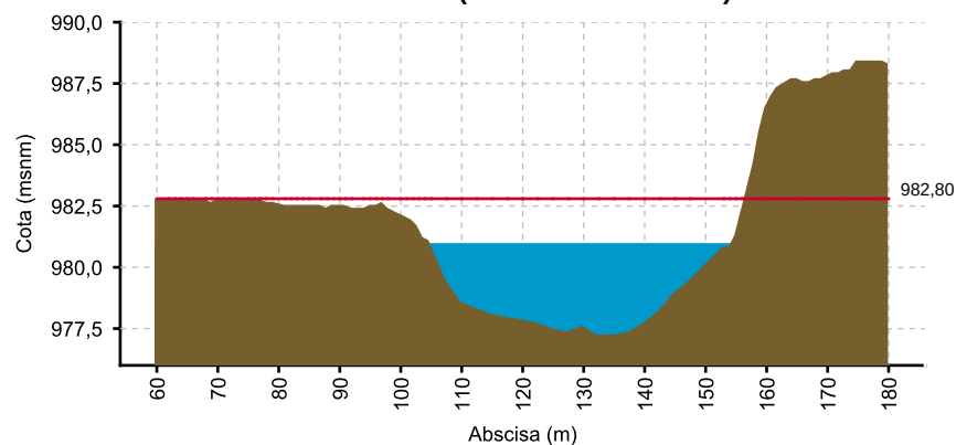
CAUCA - LA BALSA (26/04/2021 06:00 AM) NIVEL= 980.9
