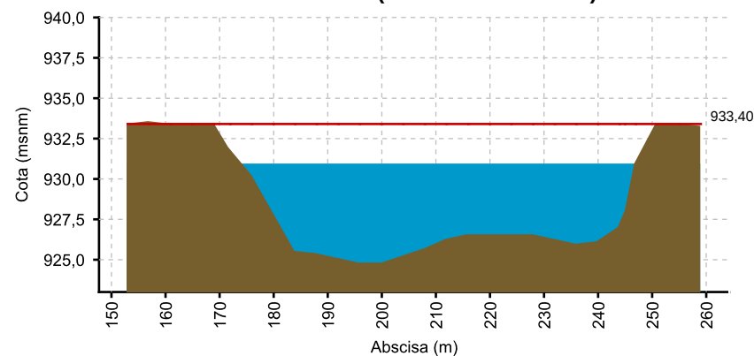
CAUCA - MEDIACANOA (28/06/2021 06:00 AM) NIVEL= 930.884
