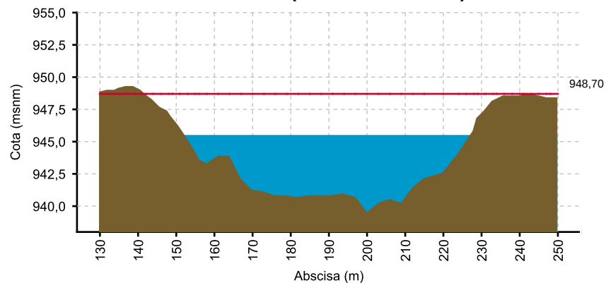
CAUCA - JUANCHITO (28/06/2021 06:00 AM) NIVEL= 945.383
